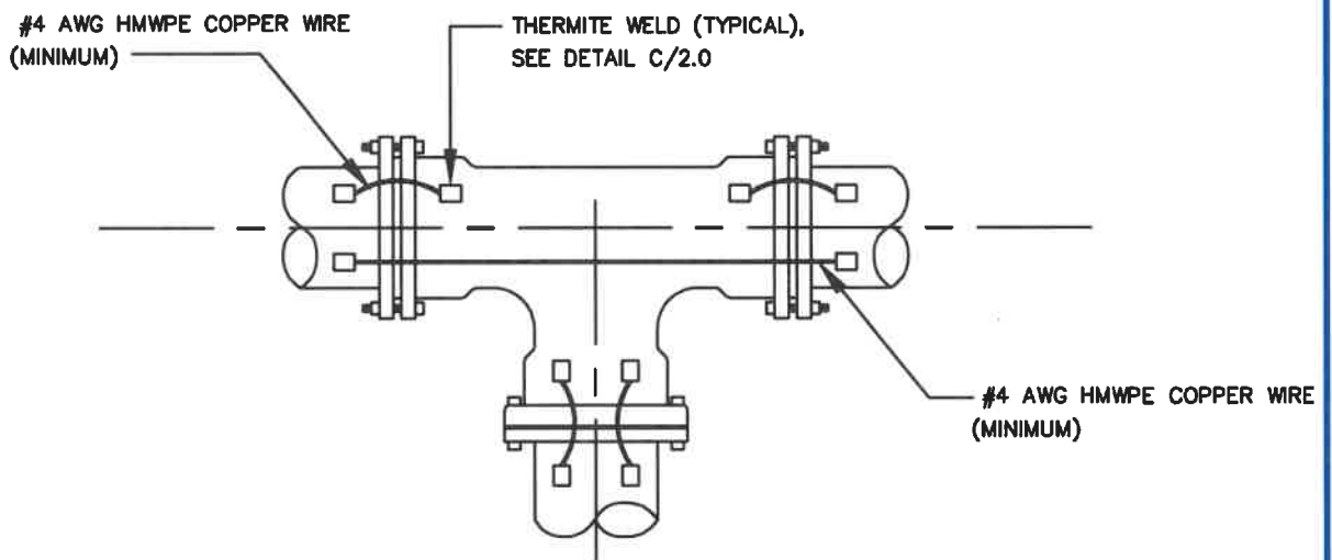
MECHANICAL JOINT TEE
