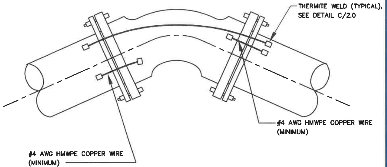
MECHANICAL JOINT BEND
