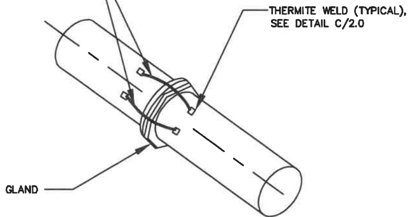
MECHANICAL JOINT
