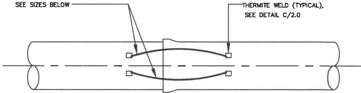
PUSH-ON JOINT
